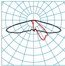
Publisca P1W-AB2L-LRA/2600-740 3G1S TX053500 DIN 5040: A30 UTE: 1,00 l CEN Flux Code: 32 69 96 100 100 0 33 67 0
