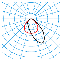
LuceoS D/H2-L CDP-A 5000-840 ETDD 03 (Ceiling D2 ZD/03+EB3) TX277138 DIN 5040: A50 UTE: 1,00 D CEN Flux Code: 60 88 97 100 100 0 0 0 0
