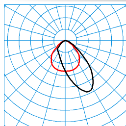
LuceoS D/H2-L CDP-A 5000-840 03 (Ceiling D2 ZD/03) TX194595 DIN 5040: A50 UTE: 1,00 D CEN Flux Code: 60 88 97 100 100 0 0 0 0
