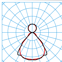
SFlow H2-L MRW LED6400-830 03 TX050991
