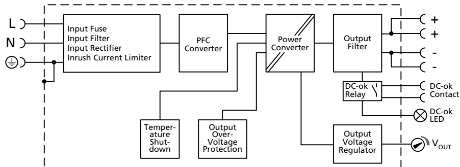
Fig. 11-1 Functional diagram
