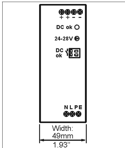
Fig. 21-1 Front view
