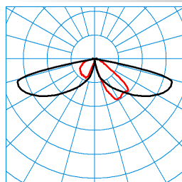
CS 19 100-AB2L-SLR1/2200-730 2G1S ET (CLO end value) TX299940 DIN 5040: A20 UTE: 1,00 l CEN Flux Code: 26 63 96 100 100 ■ C0 - C180 ■ C90 - C270
