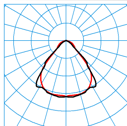
SFlow-Act C2-L MRW LED4000 ETDD8 01 (ActDWW) TX299764
