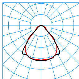
SFlow-Act C2-L MRW LED4000 ETDD8 01 (ActDCW) TX299750
