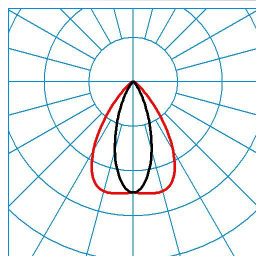
ELINE LVN180 865 L225 1 50
