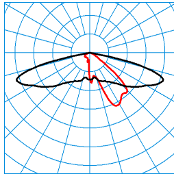
Publisca P1W-AB2L-LR/2200-740 3G1S ET (CLO initial value) TX301457 DIN 5040: A30 UTE: 1,00 l CEN Flux Code: 32 69 96 100 100 0 33 67 0
