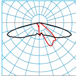
Publisca P1W-AB2L-LR/2200-740 3G1S ET (CLO end value) TX300841 DIN 5040: A30 UTE: 1,00 l CEN Flux Code: 32 69 96 100 100 0 33 67 0
