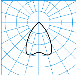
InperiaL G2 C07 BR19 1800-830 01 + RG-PC ■ C0 - C180 TX373491
