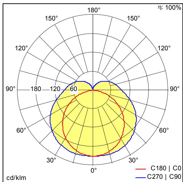
TE_ELSA_VARIOFLEX_450_800_940_FLEX1.idt
