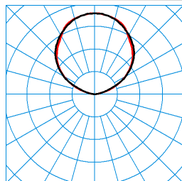
PareliaAct H-L 13000 +LM2 03 N8 (ActDWW) (LEO_indirect) TX370103 DIN 5040: E03 UTE: 0,00 J + 1,00 T CEN Flux Code: 0 0 0 0 100 48 82 97 100 ■ C0 - C180 ■ C90 - C270
