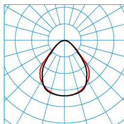
PareliaAct H-L 13000 +LM3 03 N8 (ActDCW) (LEO_direct_c270geo) TX370040 UGR I = 18,4 UGR q = 17,3 DIN 5040: A50 UTE: 1,00 C CEN Flux Code: 66 90 98 100 100 0 0 0 0 ■ C0 - C180 ■ C90 - C270
