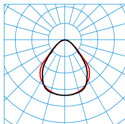
PareliaAct H-L 13000 +LM1 03 N8 (ActDWW) (LEO_direct_c270geo) TX370047
