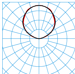
PareliaAct H-L 13000 +LM1 03 N8 (ActDSU) (LEO_indirect) TX370105 DIN 5040: E03 UTE: 0,00 J + 1,00 T CEN Flux Code: 0 0 0 0 100 48 82 97 100 ■ C0 - C180 ■ C90 - C270
