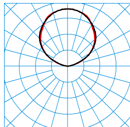
PareliaAct H-L 13000 +LM1 03 N8 (ActDCW) (LEO_indirect) TX370106 DIN 5040: E03 UTE: 0,00 J + 1,00 T CEN Flux Code: 0 0 0 0 100 48 82 97 100 ■ C0 - C180 ■ C90 - C270
