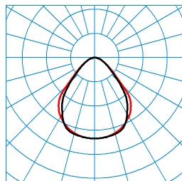
PareliaAct H-L 13000 +LM2 03 N8 (ActDCW) (LEO_direct_c90geo) TX370044 UGR I = 18,4 UGR q = 17,3 DIN 5040: A50 UTE: 1,00 C CEN Flux Code: 66 90 98 100 100 0 0 0 0 ■ C0 - C180 ■ C90 - C270
