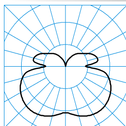
PolaroniQ W2D LED2000-840 TX373995
