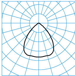
InperiaL G2 C07 BR22 2700-830 03 + ZN-PC TX052916 ■ C0 - C180
