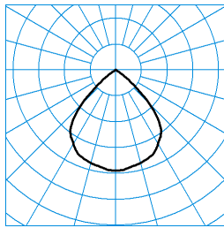
InperiaL G2 C07 BR22 2700-830 03 TX052911 ■ C0 - C180
