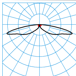
LTX Z-SB3L-LR/1500-730 2G1 TX055994
