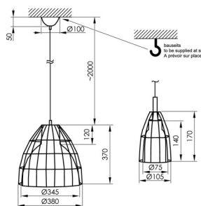
Maße [mm]
