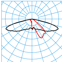
Publisca P1W-AB2L-LR/2600-740 3G1S ET (CLO end value) TX301766 DIN 5040: A30 UTE: 1,00 l CEN Flux Code: 32 69 96 100 100 0 33 67 0 ■ C0 - C180 ■ C90 - C270
