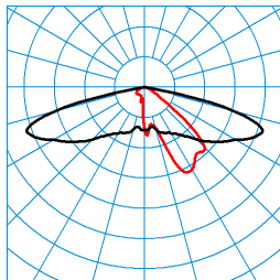
Publisca P1W-AB2L-LR/2600-740 3G1S ET (CLO initial value) TX301420 DIN 5040: A30 UTE: 1,00 l CEN Flux Code: 32 69 96 100 100 0 33 67 0 ■ C0 - C180 ■ C90 - C270
