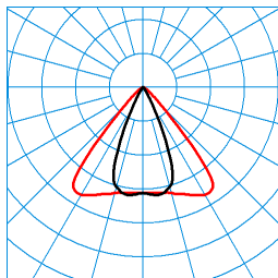
E-Line Fi Grado 30-840 J23 L37 05 (150) ■ C0 - C180 TX125314
