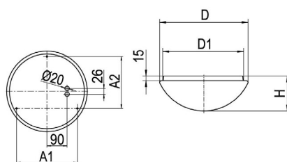
Maße [mm]
