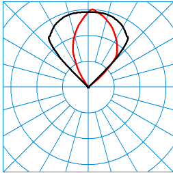
Skeo Q-W2 GT AB19R-AB19R/1600-840 (indirect) TX084371 DIN 5040: E04 UTE: 0,00 J + 1,00 T CEN Flux Code: 0 0 0 0 100 81 99 100 100
