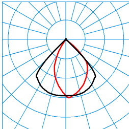
Skeo Q-W2 GT AB19R-AB19R/1600-840 (direct) TX084370 DIN 5040: A60 UTE: 1,00 B CEN Flux Code: 81 99 100 100 100
