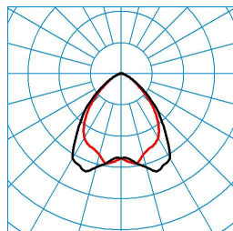
ELINE HE LW100 827-65 L225 4 50
