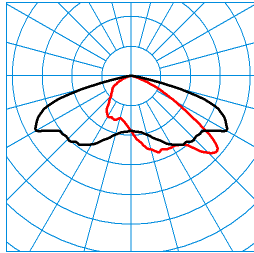
LIQ 70N-AB7L-LRA/6800-727 8G1 ETDD(CLO initial value) TX278338 DIN 5040: A30 UTE: 1,00 G CEN Flux Code: 35 73 98 100 100 0 0 0 0
