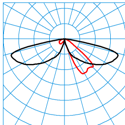
LTX P-AB2L-LRA/15/18/26-740 4G1 (1500 lm) TX059699 DIN 5040: A20 UTE: 1,00 l CEN Flux Code: 24 61 92 100 100 0 0 0 0 ■ C0 - C180 ■ C90 - C270
