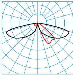
LTX P-AB2L-LRA/15/18/26-740 4G1 (1800 lm) TX062701 DIN 5040: A20 UTE: 1,00 l CEN Flux Code: 24 61 92 100 100 0 0 0 0 ■ C0 - C180 ■ C90 - C270
