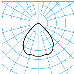
InperiaL G2 C07 BR22 1800-830 03 + RD-PC TX373582 ■ C0 - C180
