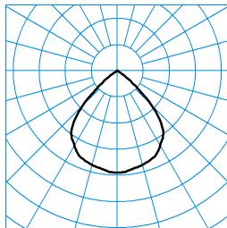
InperiaL G2 C07 BR22 1800-830 03 TX373585 ■ C0 - C180
