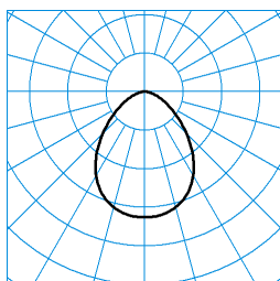
InperiaL G2 C07 BR22 1800-830 03 + DA-M 03 TX373583 ■ C0 - C180
