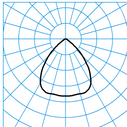
InperiaL G2 C07 BR22 1800-830 03 + ZN-PC TX373580 ■ C0 - C180
