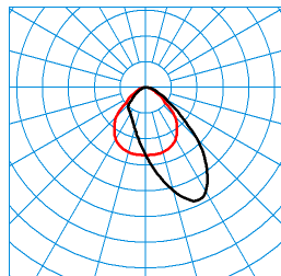
LuceoS D/H2-L CDP-A 6500-830 03 (Pendant ZS/ZST) TX194612 DIN 5040: A50 UTE: 1,00 D CEN Flux Code: 60 88 97 100 100 0 0 0 0
