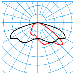
LIQ 70N-AB7L-SLR1/7500-727 8G1 ET (CLO end value) TX278196 DIN 5040: A30 UTE: 1,00 G CEN Flux Code: 35 73 98 100 100 0 0 0 0 ■ C0 - C180 ■ C90 - C270
