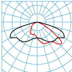
LIQ 70N-AB7L-SLR1/7500-727 8G1 ET (CLO initial value) TX278269 DIN 5040: A30 UTE: 1,00 G CEN Flux Code: 35 73 98 100 100 0 0 0 0 ■ C0 - C180 ■ C90 - C270
