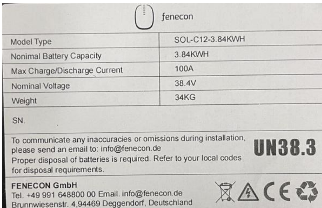
Fig.5 – Label view of Battery
