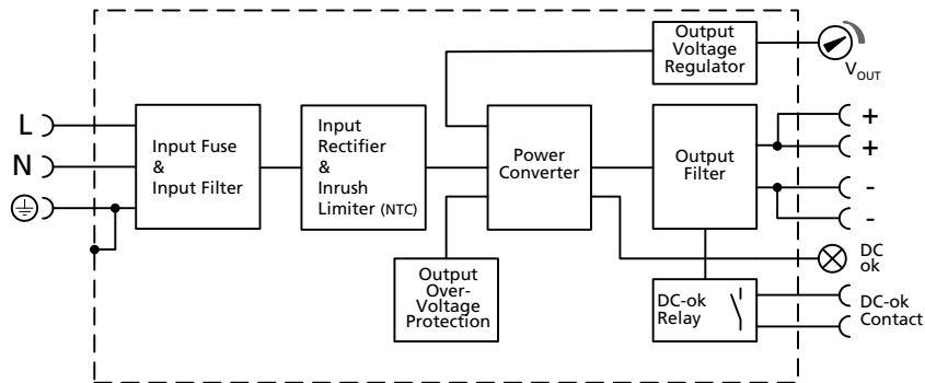
Fig. 11-1 Functional diagram PIC240.241C
