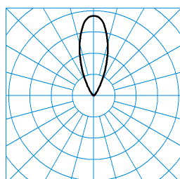
Altigo G2 120 WO RB17L/3800-830 1G1P + VE IP66 24V DC 130W TX120453 ■ C0 - C180
