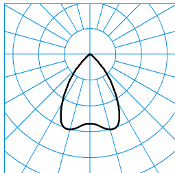
InperiaL G2 C07 BR25 4700-830 01 + RG-PC ■ C0 - C180 TX373456
