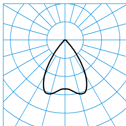
InperiaL G2 C07 BR25 4700-830 01 + ZN-PC ■ C0 - C180 TX373454
