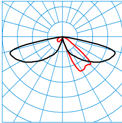
LTX P-AB2L-LRA/15/18/26-730 4G1 (2600 lm) TX062700 DIN 5040: A20 UTE: 1,00 l CEN Flux Code: 24 61 92 100 100 0 0 0 0 ■ C0 - C180 ■ C90 - C270
