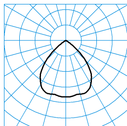
InperiaL G2 C07 BR22 2700-840 03 + RG-PC ■ C0 - C180 TX373340
