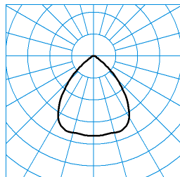
InperiaL G2 C07 BR22 2700-840 03 + ZN-PC ■ C0 - C180 TX373339
