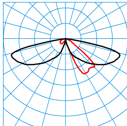
LTX K-AB2L-LRA/15/18/26-740 4G1 (2600 lm) TX062694 DIN 5040: A20 UTE: 1,00 l CEN Flux Code: 24 61 92 100 100 0 0 0 0 ■ C0 - C180 ■ C90 - C270
