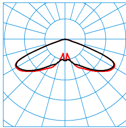
Publisca P2-RB6L-LRA/5600-740 6G1S TX047915
