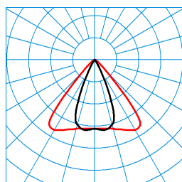
E-Line Fi Grado 30-830 J21 L37 01 (225) ■ C0 - C180 ■ C90 - C270 TX123657
