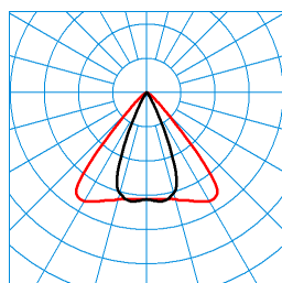
E-Line Fi Grado 50-840 J23 L37 01 (225) ■ C0 - C180 TX123814
