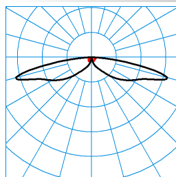
LTX P-SB3L-LR/1500-740 2G1 TX055943
