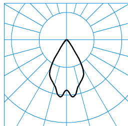
InperlaLP C05 BR19 1000-830 03 + ZN-PC TX369709 ■ C0 - C180
