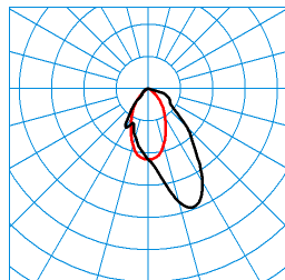
CreavoAct M48-TS LWW-03 53-8 ETDD8 01(CTDCW) TX195453 ■ C0 - C180 ■ C90 - C270 DIN 5040: A50 UTE: 1,00 C CEN Flux Code: 70 92 99 100 100
