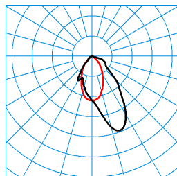
CreavoAct M48-TS LWW-03 53-8 ETDD8 01(CTDSU) TX195454 ■ C0 - C180 ■ C90 - C270 DIN 5040: A50 UTE: 1,00 C CEN Flux Code: 70 92 99 100 100
