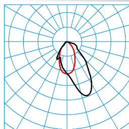
CreavoAct M48-TS LWW-03 53-8 ETDD8 01(CTDWW) TX195455 ■ C0 - C180 ■ C90 - C270 DIN 5040: A50 UTE: 1,00 C CEN Flux Code: 70 92 99 100 100
