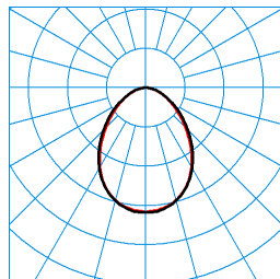
SFlow C2-L MRWD LED4000-830 01 TX050951
