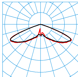
Publisca P1W-RB6L-LR/2600-740 3G1S ET (CLO end value) TX300998 DIN 5040: A20 UTE: 1,00 J CEN Flux Code: 19 57 99 100 100 0 50 50 0
