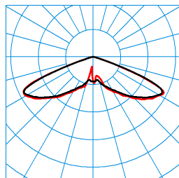
Publisca P1W-RB6L-LR/2600-740 3G1S ET (CLO initial value) TX301719 DIN 5040: A20 UTE: 1,00 J CEN Flux Code: 19 57 99 100 100 0 50 50 0
