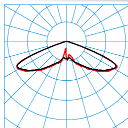
Publisca P1W-RB6L-LR/2600-740 3G1S TX053532 DIN 5040: A20 UTE: 1,00 J CEN Flux Code: 19 57 99 100 100 0 50 50 0
