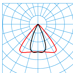
E-Line Fi Grado 50-830 J21 L37 05 (225) TX372274 ■ C0 - C180 ■ C90 - C270 UGR I = 28,0 UGR q = 12,0 DIN 5040: A70 UTE: 0,93 A CEN Flux Code: 92 99 100 100 93
