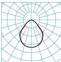
Parelia H-L 13000-840 +LM1 +LLWS 03 (direct c270geo) TX059613
