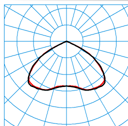
E-Line Fi L-SHB 24V Inotec L37 01 (150) TX125328
