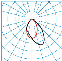
CreavoAct D3-L LWW-03 41-8 ETDD8 01(ACDSU) TX278556 ■ C0 - C180 ■ C90 - C270 DIN 5040: A50 UTE: 1,00 B CEN Flux Code: 71 94 99 100 100
