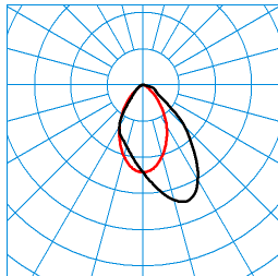
CreavoAct D3-L LWW-03 41-8 ETDD8 01(ACDCW) TX278553 ■ C0 - C180 ■ C90 - C270 DIN 5040: A50 UTE: 1,00 B CEN Flux Code: 71 94 99 100 100
