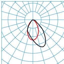
CreavoAct D3-L LWW-03 41-8 ETDD8 01(ACDWW) TX278533 ■ C0 - C180 ■ C90 - C270 DIN 5040: A50 UTE: 1,00 B CEN Flux Code: 71 94 99 100 100
