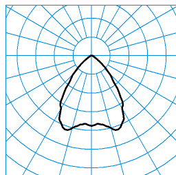
InperiaLP C05 BR22 1000-830 03 + RG-PC TX374000 ■ C0 - C180
