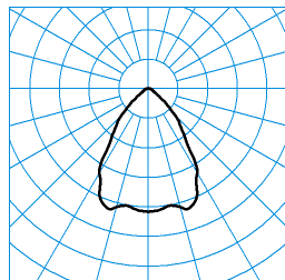
InperiaLP C05 BR22 1000-830 03 + ZN-PC TX373999 ■ C0 - C180
