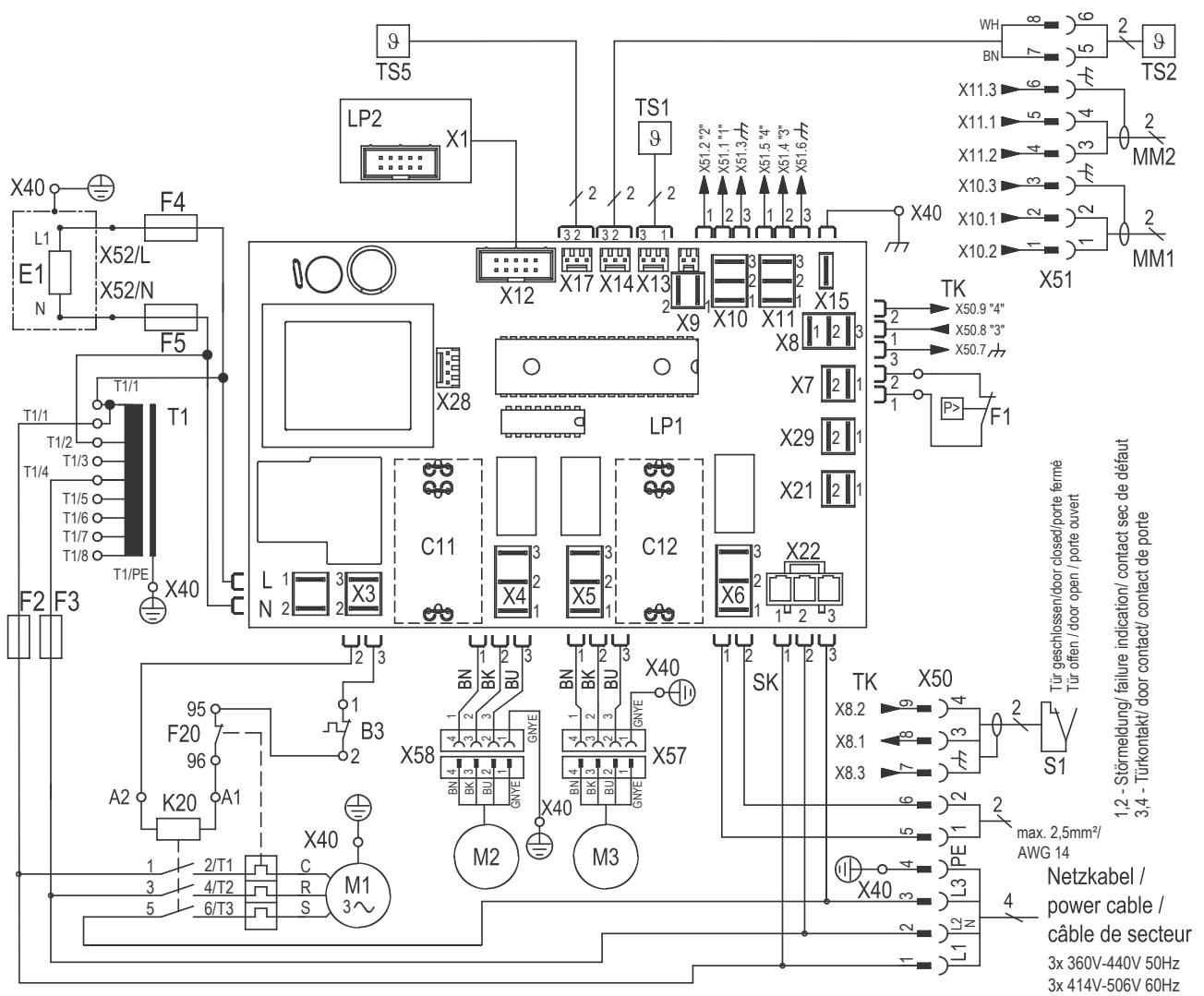
Fig. 21: Circuit diagram
