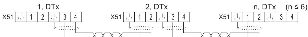
Fig. 22: Control Multimaster
