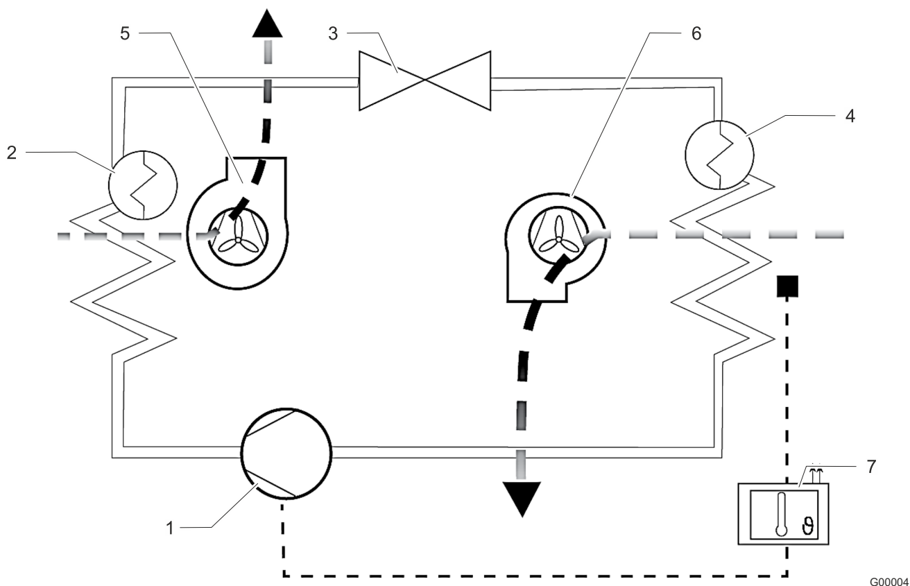
Fig. 7: circuit frigorifique
