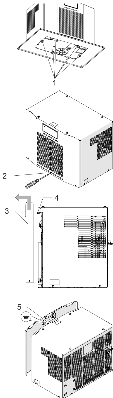
Fig. 17: Removing the front flap
