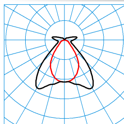
TugraHE+ 15 PW19 50-840 ETDD 01 TX303475
