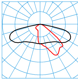
Cuvia 40-AB2L-LR/3200-740 4G1S TX046945
