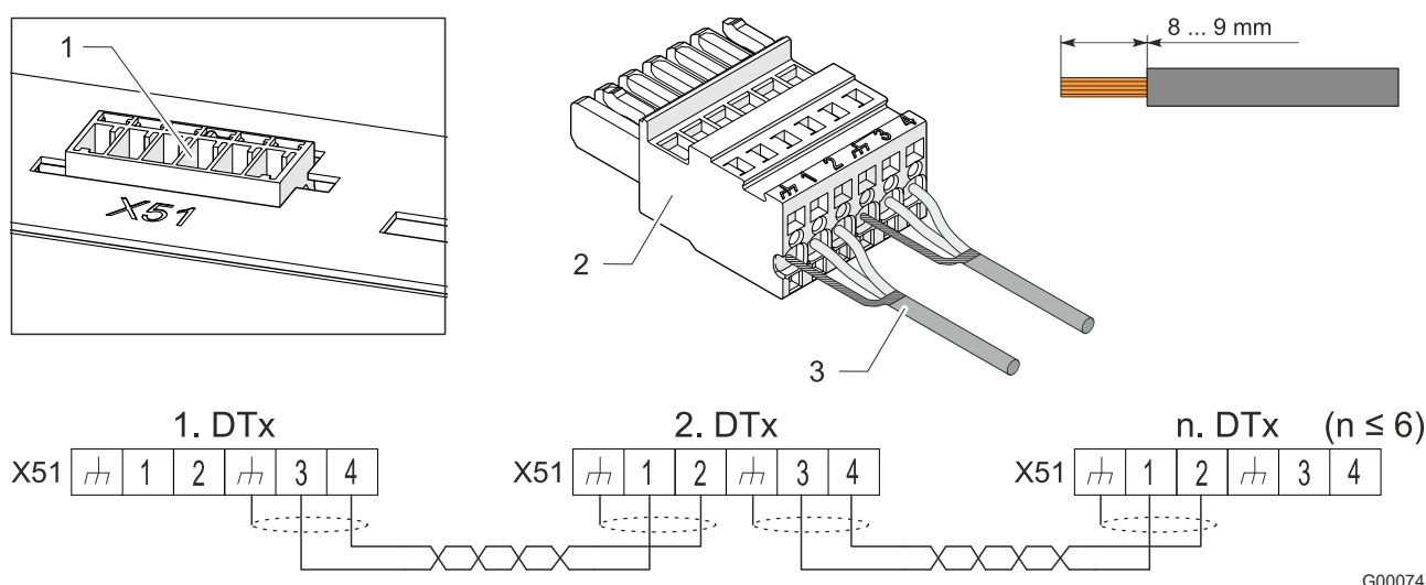
Fig. 17: Controllo Multimaster
