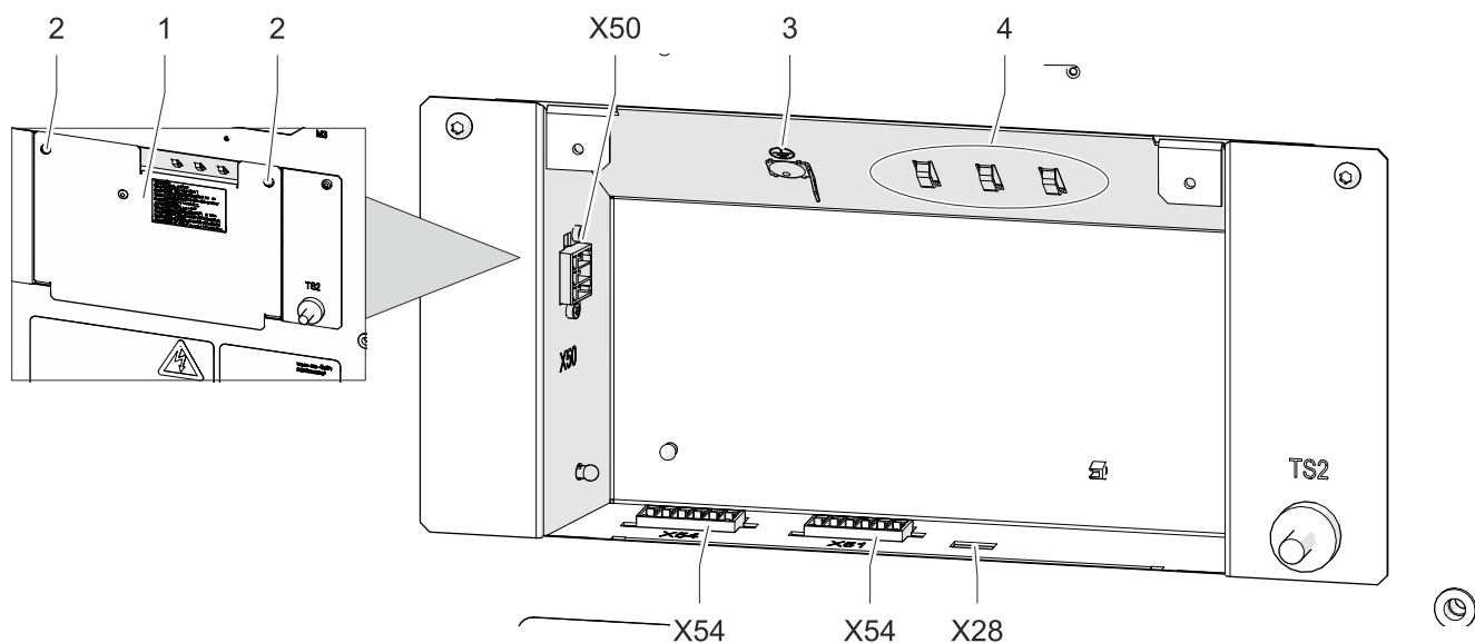
Fig. 16: Connection compartment
