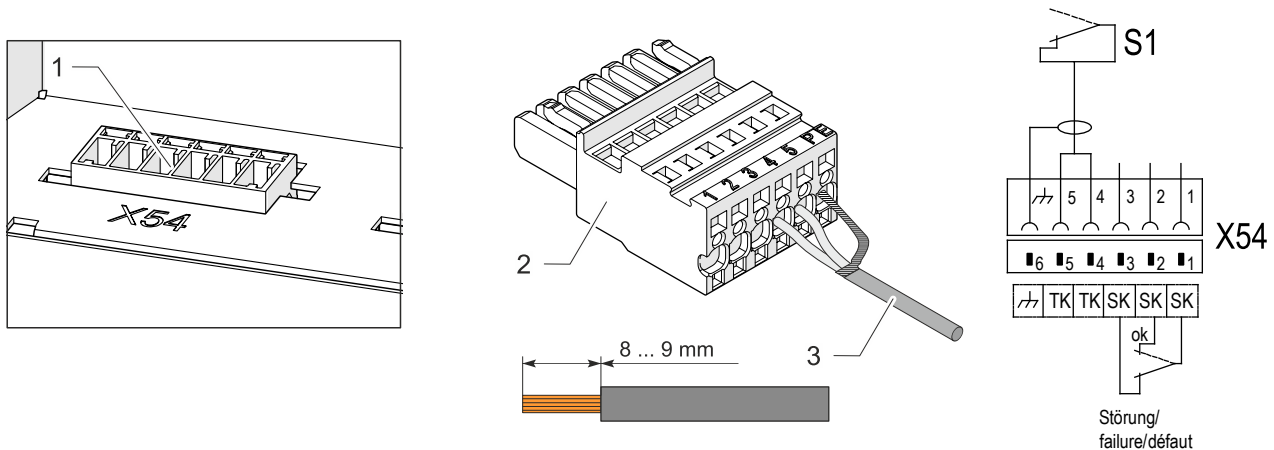
Fig. 18: Connecting a door contact switch
