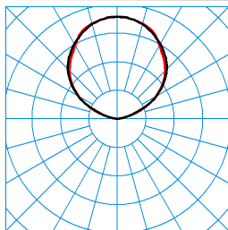
PareliaAct H-L 13000 +LM2 +LLWS 03 N8 (ActDWW) (LEO_indirect) TX370112
