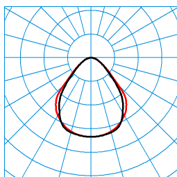
PareliaAct H-L 13000 +LM3 +LLWS 03 N8 (ActDCW) (LEO_direct_c270geo) TX370065
