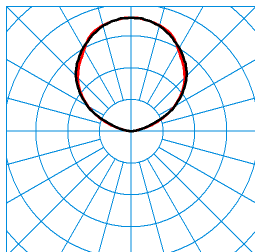
PareliaAct H-L 13000 +LM3 +LLWS 03 N8 (ActDCW) (LEO_indirect) TX370114
