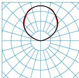
PareliaAct H-L 13000 +LM3 +LLWS 03 N8 (ActDSU) (LEO_indirect) TX370113
