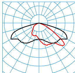
LIQ 70N-AB7L-LR/9100-722 10G1 ET (CLO initial value) TX280903 DIN 5040: A30 UTE: 1,00 G CEN Flux Code: 35 73 98 100 100 0 0 0 0 ■ C0 - C180 ■ C90 - C270
